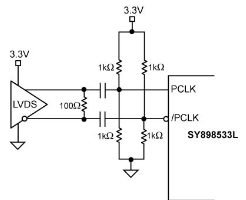
Figure 3f. LVDS Interface (AC-Coupled)
